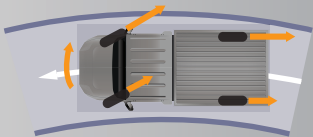
ELECTRONIC BRAKE- FORCE DISTRIBUTION (All High Type)
